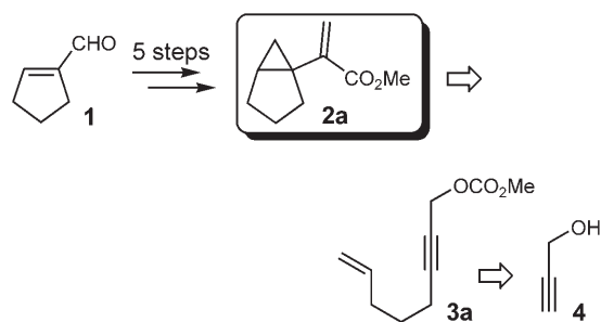
Scheme 1. Previous [5] and newly conceived synthesis of methyl 2-(bicyclo[3.1.0]hex-1-yl)acrylate.
