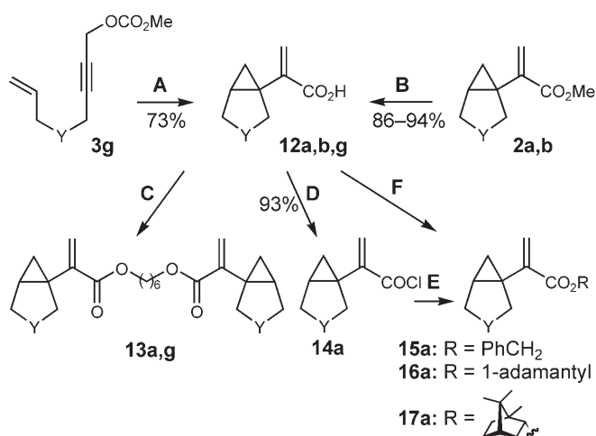
Scheme 7. Representative examples for modification of bicyclic acrylic acids 12a and g : A : 3 mol % \text{Pd}(\text{OAc})_2 , 2.2 \text{P}(2\text{-furyl})_3 , 1.1 \text{Me}_4\text{NBr} , 1.1 BHT (equivalents with respect to Pd), 60% aqueous \text{AcOH} , 1 bar \text{CO} , 25 °C, 24 h. B : \text{LiOH} \cdot \text{H}_2\text{O} , 70% aqueous acetone, 25 °C, 24 h. C : 1,6-Hexanediol, \text{PPh}_3 , DEAD, THF, –70 to 25 °C, 3 h. D : (\text{COCl})_2 , \text{CH}_2\text{Cl}_2 , DMF, 25 °C, 3 h. E : Alcohol, \text{NEt}_3 , DMAP, \text{CH}_2\text{Cl}_2 , 25 °C, 36 h. F : Benzyl chloride, \text{K}_2\text{CO}_3 , KI, DMF, 25 °C, 24 h. For yields of esters 13 and 15–17 see the Table 5.
