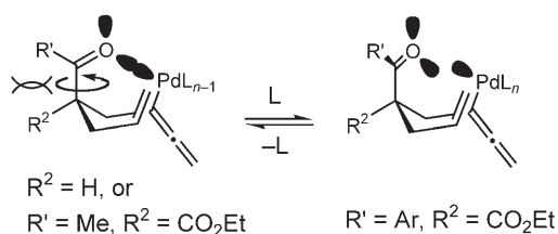
Scheme 6. Stereoelectronic aspects of the ring-closure step of 1,6-enyne precursors 3c , d , f and h-j with two different substituents in the tether.
