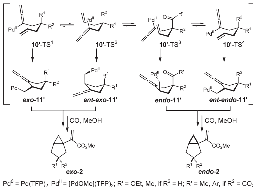
Scheme 5. Stereochemical aspects of the palladium-catalyzed cascade bicyclization.
