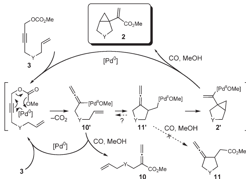
Scheme 4. General catalytic cycle for Pd-catalyzed cycloisomerization-carbonylation cascades of alkenyl-tethered propargyl carbonates.
