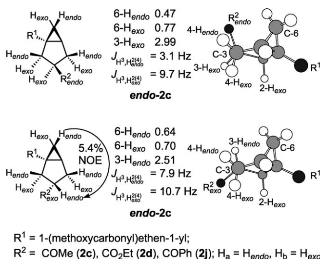
Figure 1. Assignment of the relative configuration of the diastereomeric 3-acylbicyclo[3.1.0]hexylacrylates 2c , d and j .
